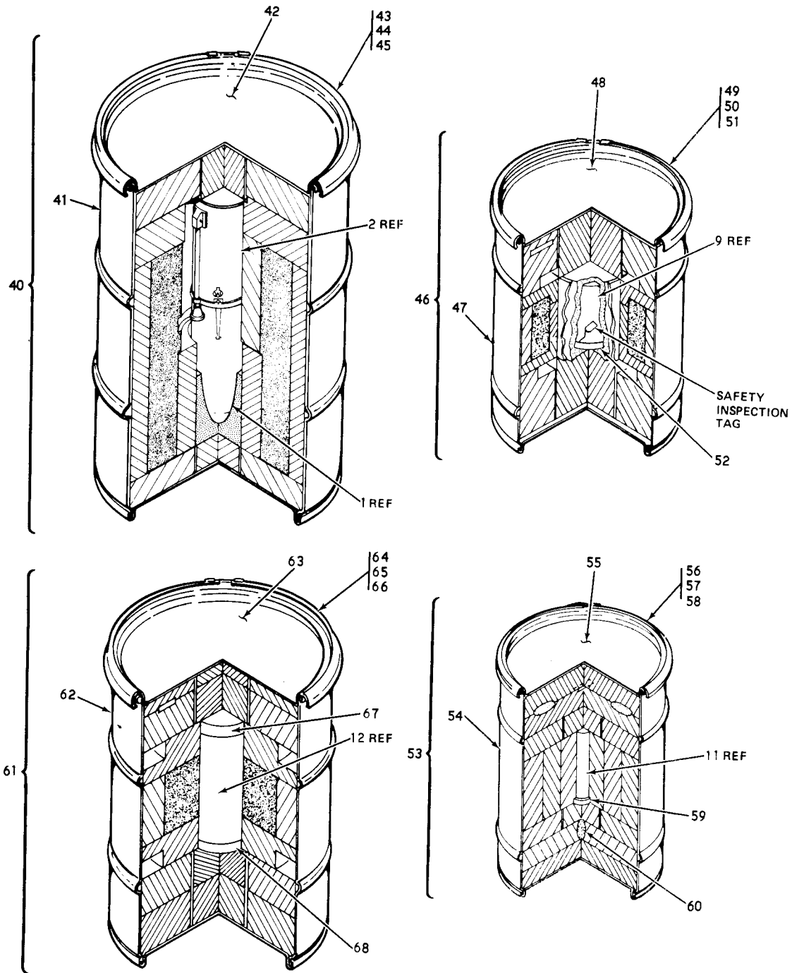
Figure 1. (Group 0100) Intercept-aerial guided missile MIM-72A (1569726), MIM-72B (Training) (2604974), MIM-72D (10234562) - partial exploded view - Sheet 3 of 4.
