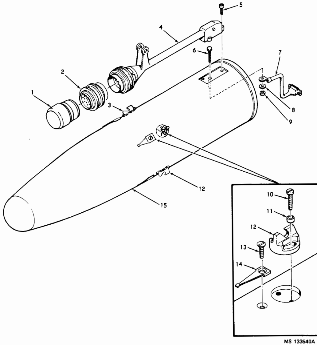
Figure 13. (Group 0620) Command guidance control group Training (2603341) - partial exploded view
