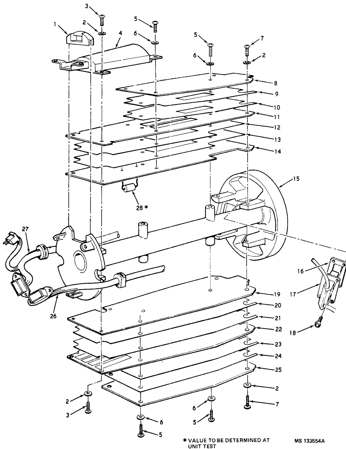
Figure 4. (Group 0125) Electronics Section (2604715 Mod 1, 2605664 Mod 2, 1569576 Mod 0) - exploded view
