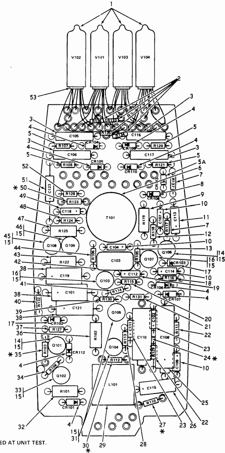
Figure 7. (Group 0140) Gyro drive amplifier (1569583)
