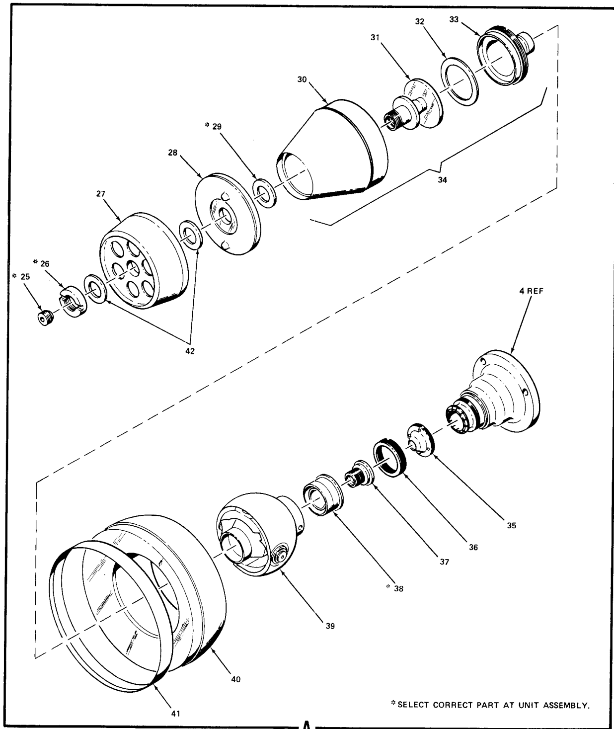
Figure 3. (Group 0115) Guided Missile infrared seeker section (2603654) - partial exploded view - Sheet 2 of 2
