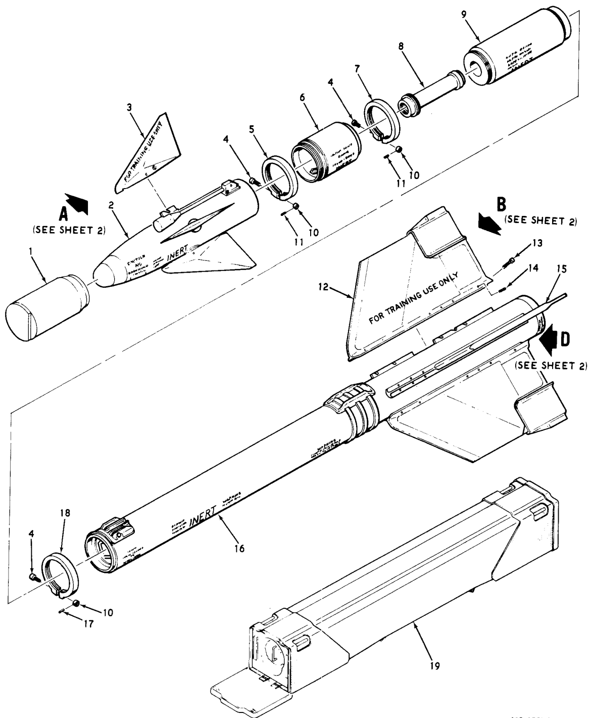
Figure 12. (Group 0600) M-30 guided missile training (1569729) - partial exploded view - Sheet 1 of 2
