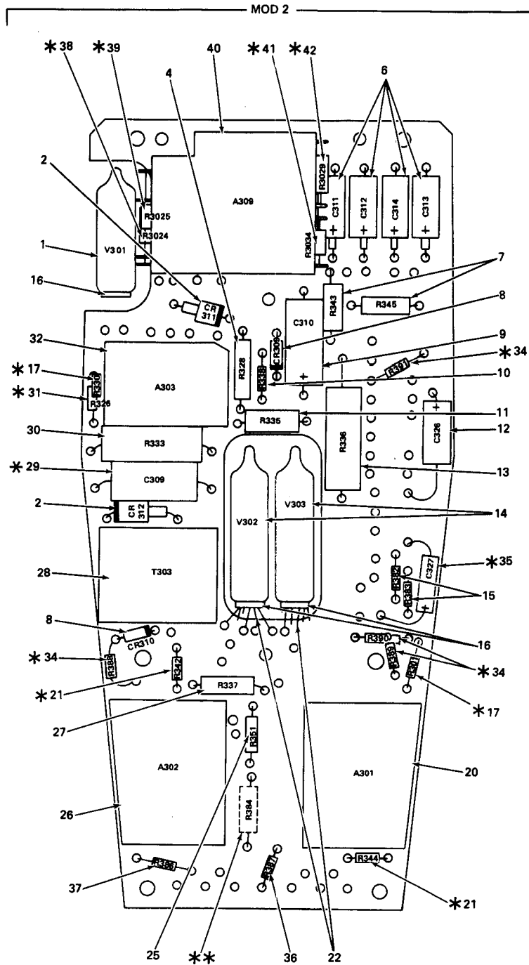
Figure 6. (Group 0135) Caging Amplifier (1569577-MOD 0, 2604716-MOD 1, or 2605662-MOD 2)- Sheet 3 of 3
