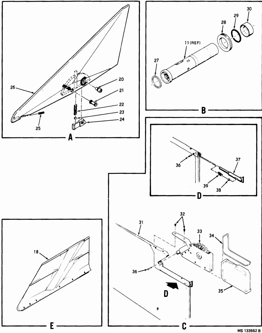
Figure 1. (Group 0100) Intercept-aerial guided missile MIM-72A (1569726), MIM-72B (Training) (2604974), MIM-72D (10234562) - partial exploded view - Sheet 2 of 4
