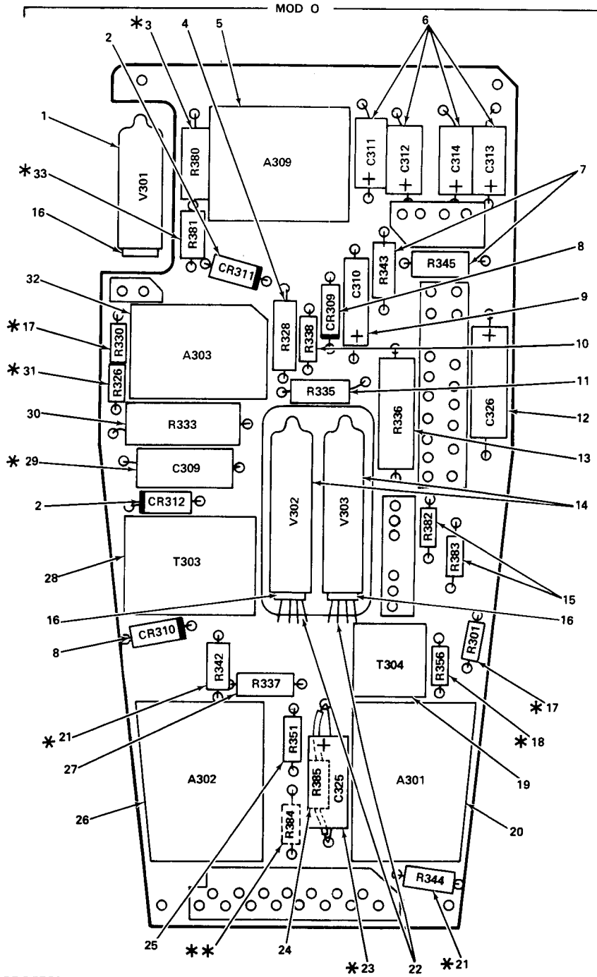
Figure 6. (Group 0135) Caging Amplifier (1569577-MOD 0, 2604716-MOD-1, or 2605662-MOD-2) - Sheet 1 of 3
