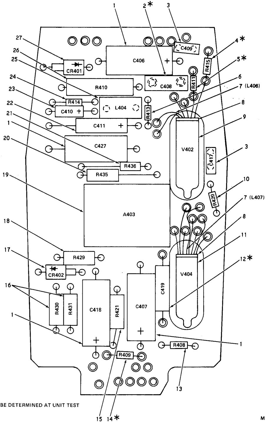
Figure 5. (Group 0130) Carrier amplifier (1569586)
