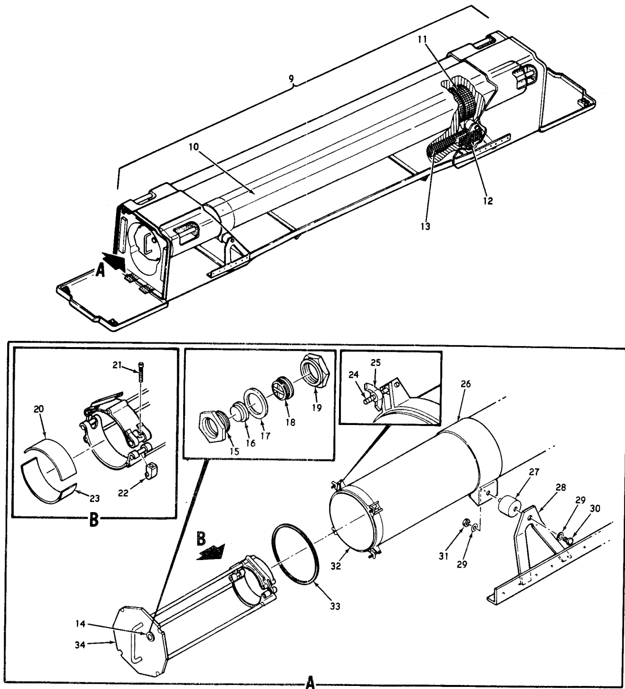
Figure 17. (Group 1000) M-570 Guided missile shipping and storage container (11074804) - partial exploded view - Sheet 2 of 2
