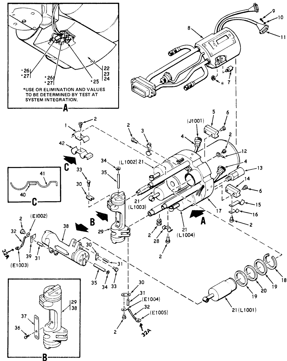
Figure 9. (Group 0150) Servo section (1569571) - exploded view
