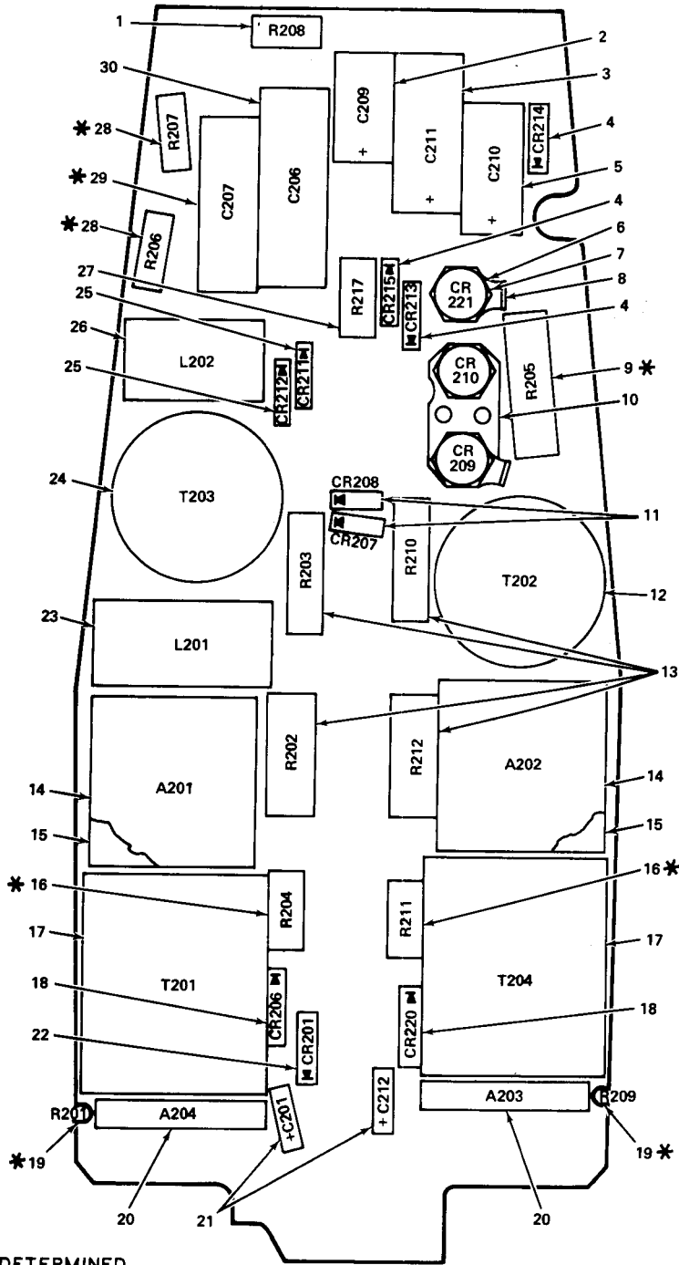
Figure 8. (Group 0145) Magnetic amplifier (1569861)
