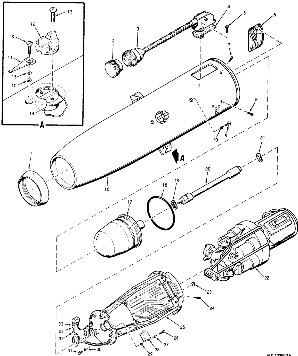
Figure 2. (Group 0110) Guidance section (1569570, 2604720, or 2605665) - partial exploded view
