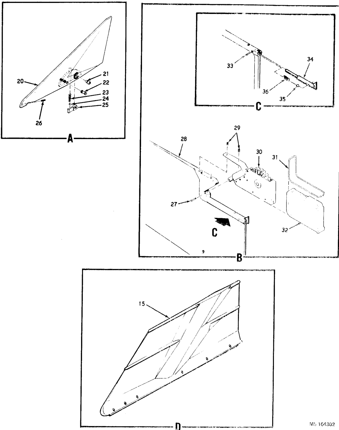
Figure 12. (Group 0600) M-30 Guided Missile Training (1569729)-partial exploded view - Sheet 2 of 2
