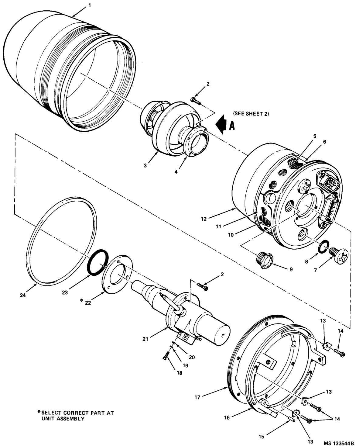
Figure 3. (Group 0115) Guided missile infrared seeker section (2603654) -partial exploded view - Sheet 1 of 2
